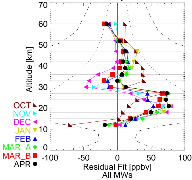
HNO3 REC analysis - Altitude
