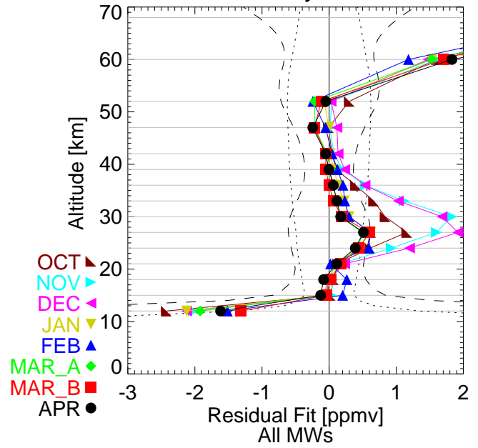
N2O REC analysis - Altitude
