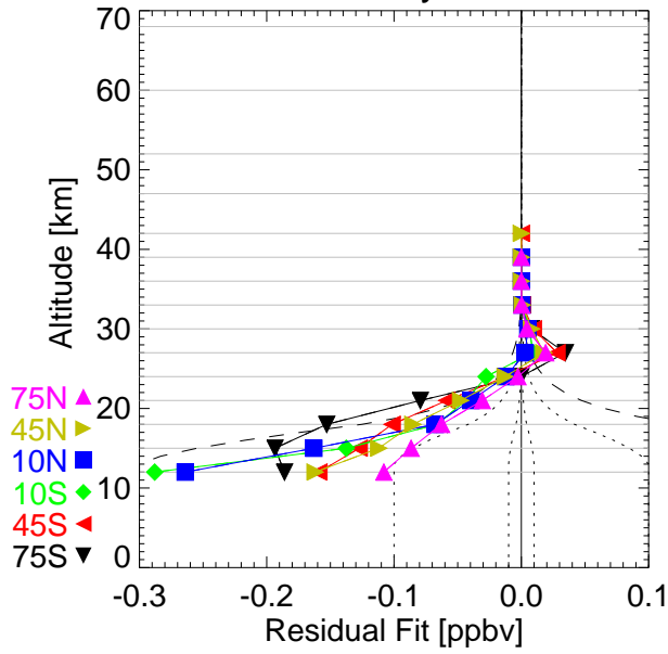
NH3 REC analysis OCT02
