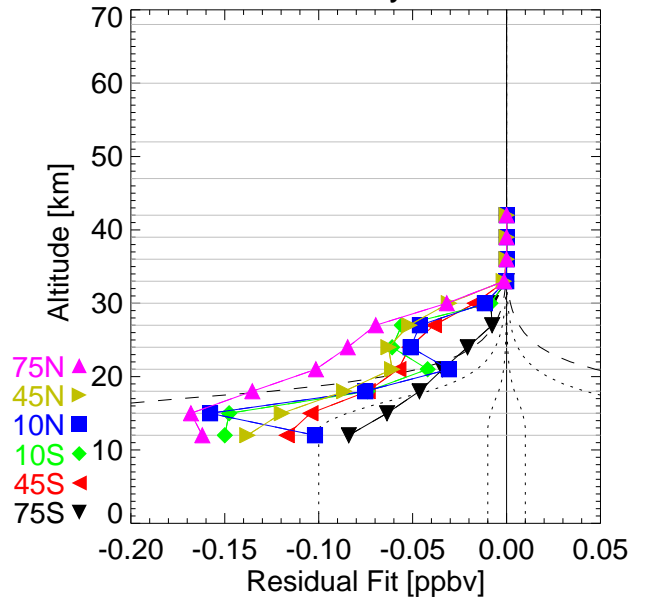
NH3 REC analysis MAY03
