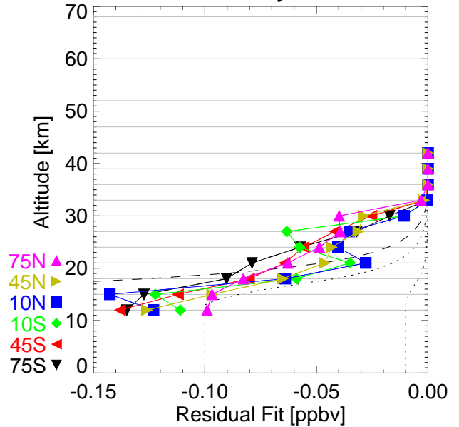
NH3 REC analysis MAR03
