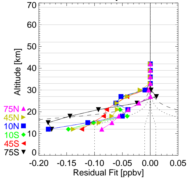
NH3 REC analysis NOV02
