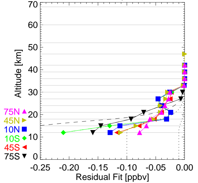
NH3 REC analysis JAN03
