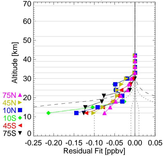
NH3 REC analysis DEC02
