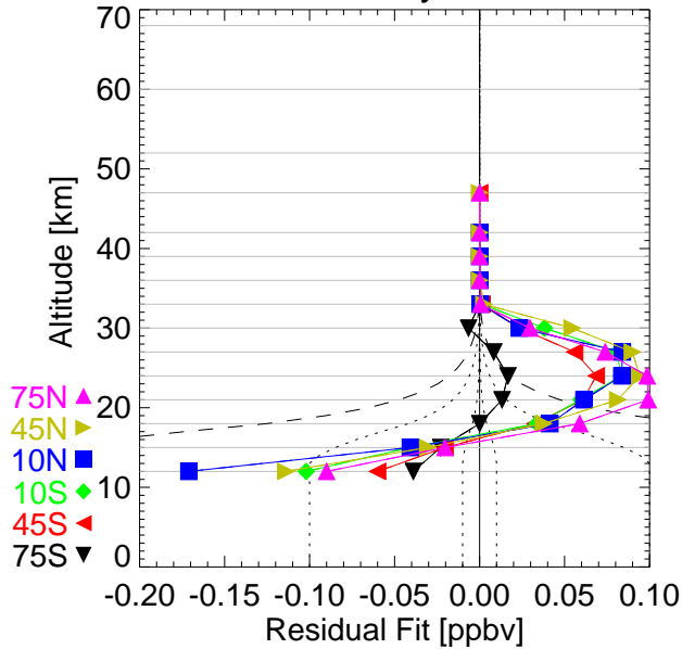
NH3 REC analysis AUG03
