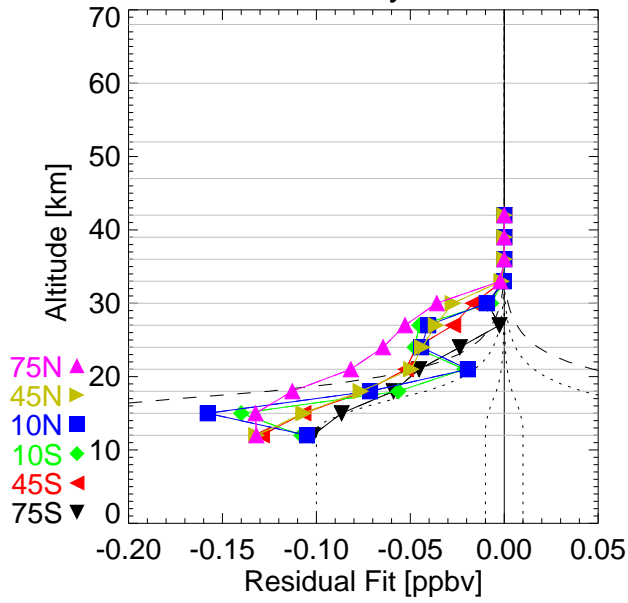
NH3 REC analysis APR03
