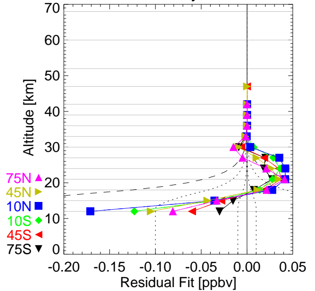
NH3 REC analysis SEP03
