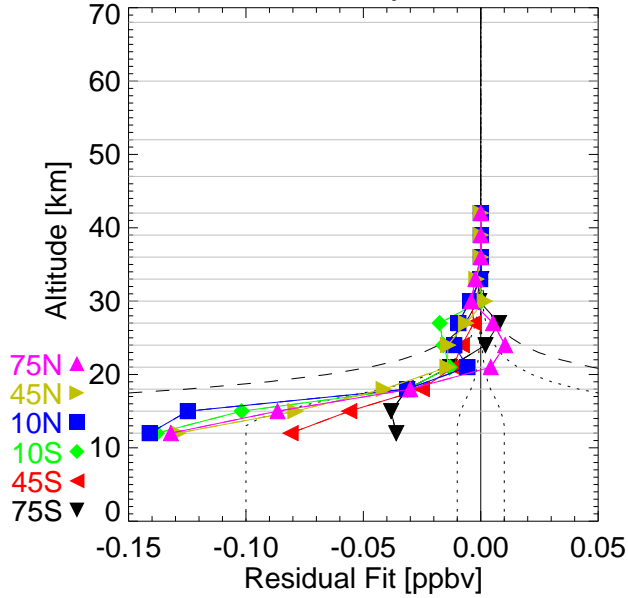
NH3 REC analysis JUN03
