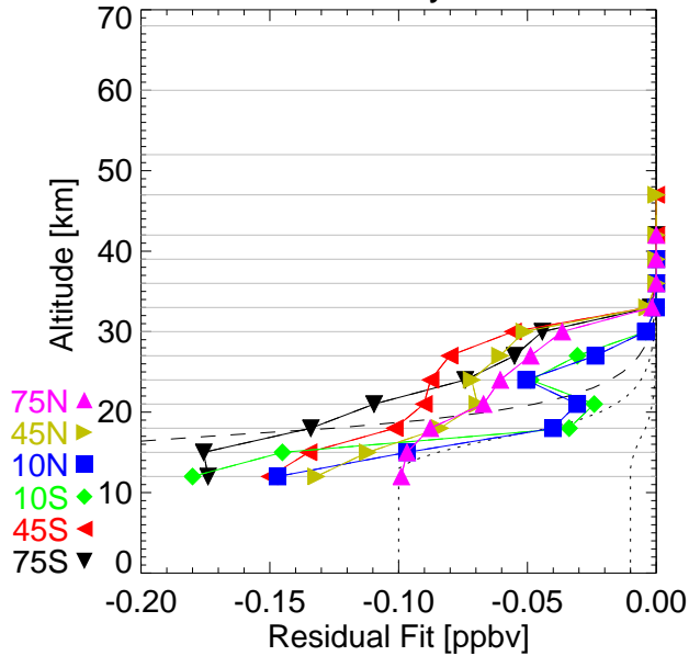
NH3 REC analysis FEB03
