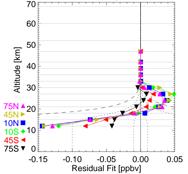
NH3 REC analysis JUL03
